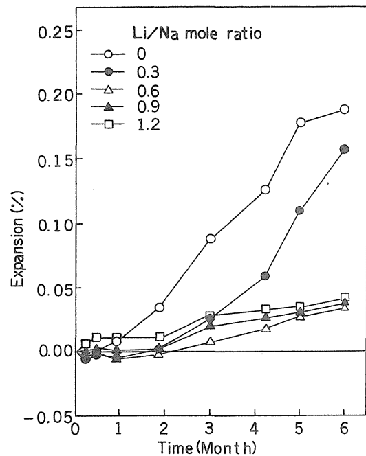
Fig. 1. Expansion of mortars adding LiNO 2 stored in a fog box at 40°C.
