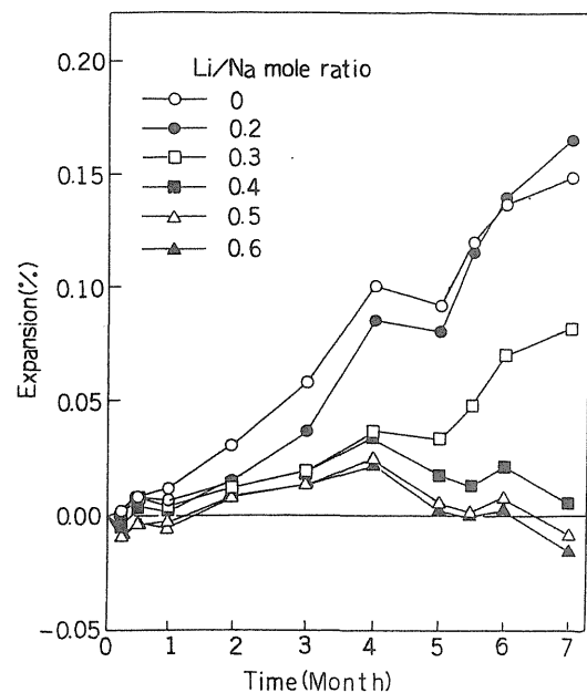
Fig. 2. Detailed expansion behaviors of mortars adding LiNO 2 stored in a fog box at 40°C.
